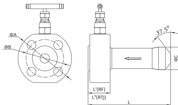
Needle Valve
