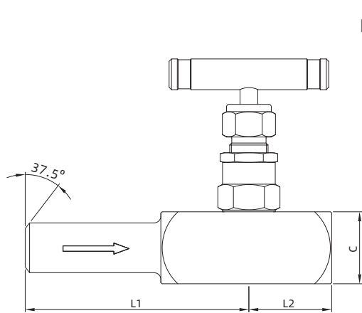
Needle Valve
