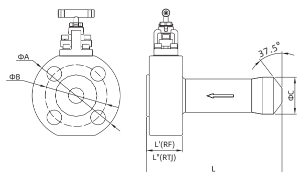
OS&Y Needle Valve
