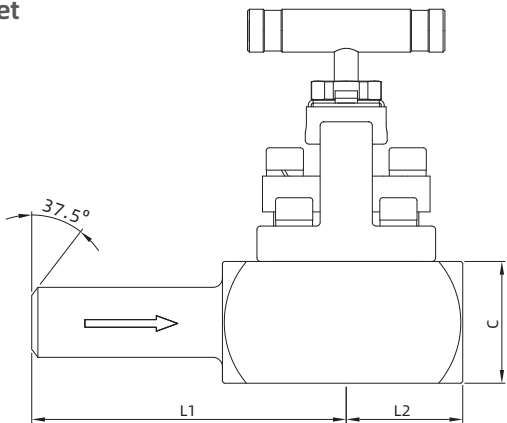
OS&Y Needle Valve
