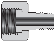
Thread to Pipe Unions (TPU)
