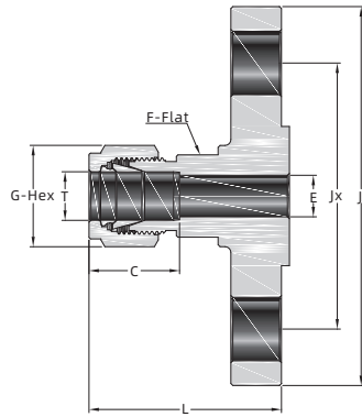
DIN/GB Flanges, Pressure Class PN 40
