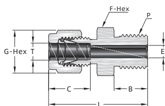
Fractional Tube
