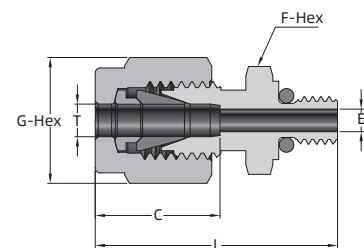
Fractional Tube
