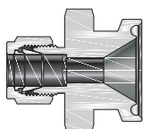
Sanitary Flange Fittings
