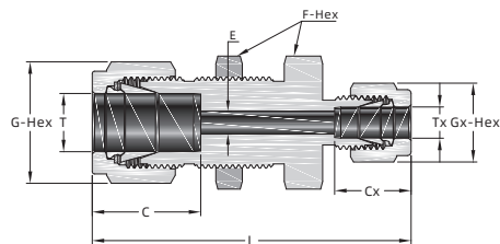
Fractional Tube
