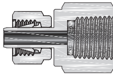
1 1/4" and above
