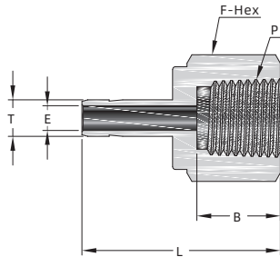
1" and below
