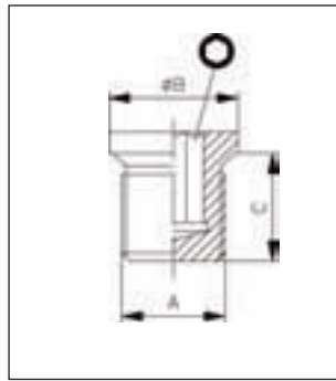
Zátka DIN 908 Parallel male plug
